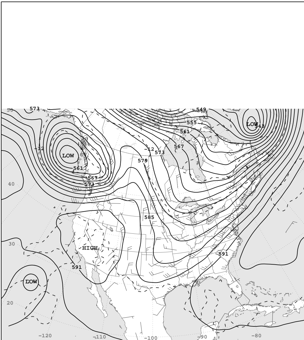
TUE, JUL 23, 2024 500-Millibar Height Contours at 7:00 A.M. E.S.T.
