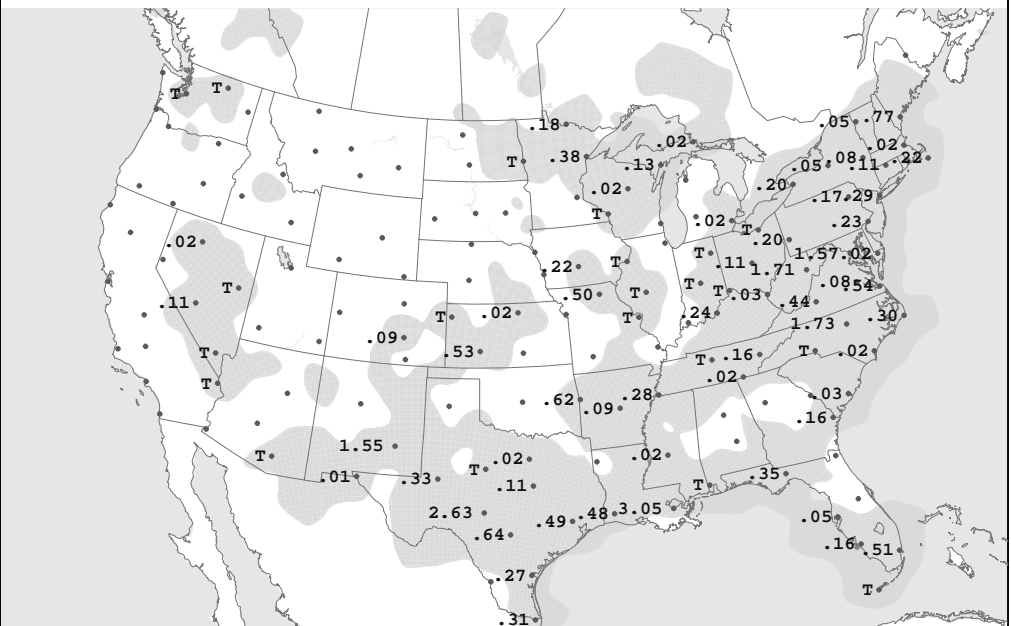
TUE, JUL 23, 2024 24-hour Precipitation Areas and Amounts Ending 7:00 A.M. E.S.T.
