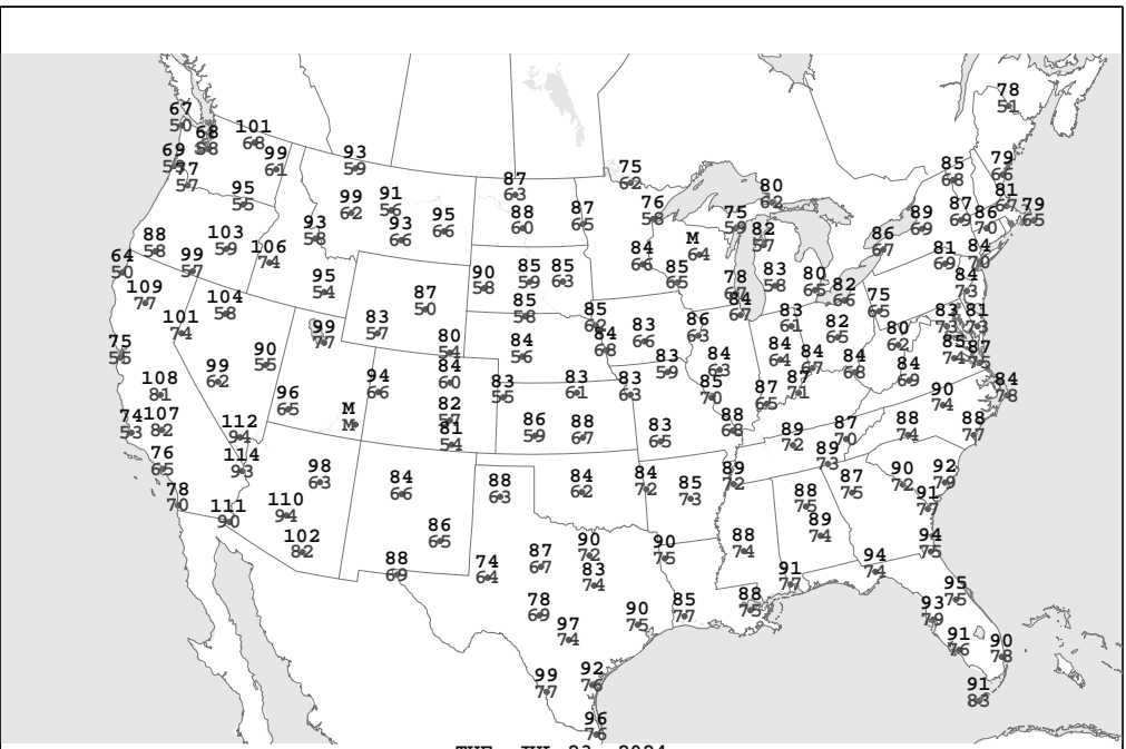
TUE, JUL 23, 2024 Highest and Lowest Temperature
