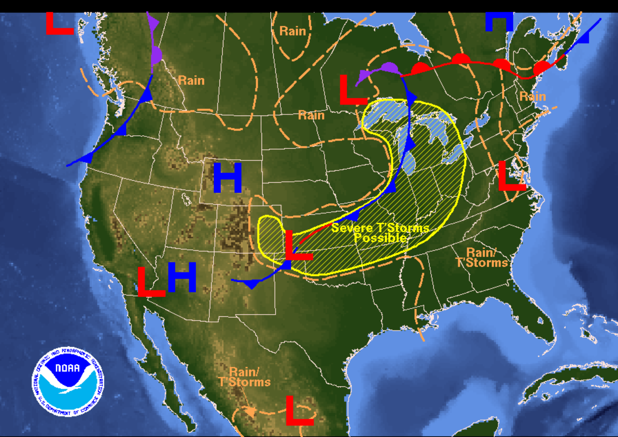
Weather Forecast for Thursday, June 30, 2005 DOC/NOAA/NWS/NCEP/Hydrometeorological Prediction Center Prepared by Fries/Oravec based on HPC, SPC, and TPC forecasts.
