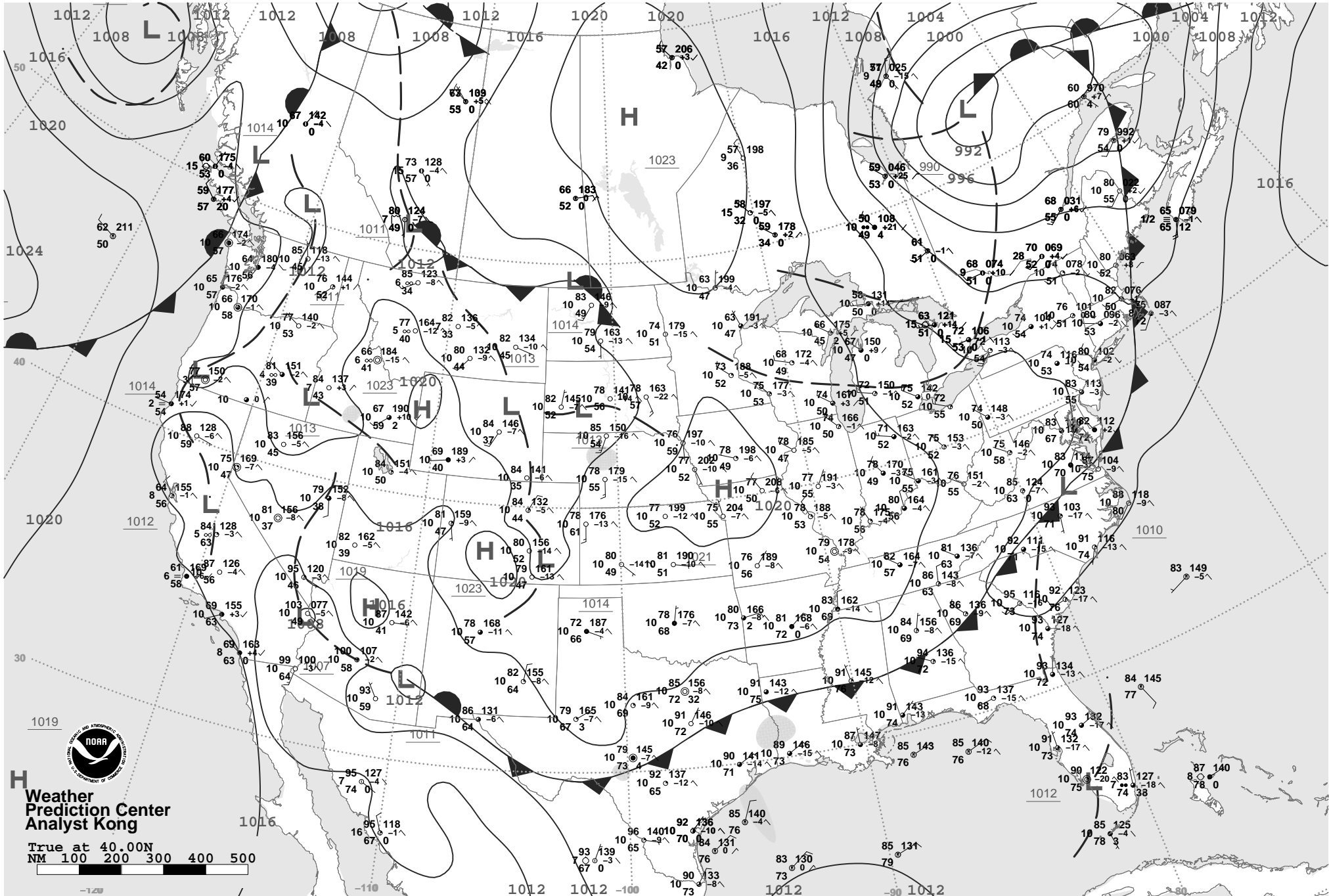
WED AUG 23 2017 18 UTC Surface Weather Map and Station Weather
