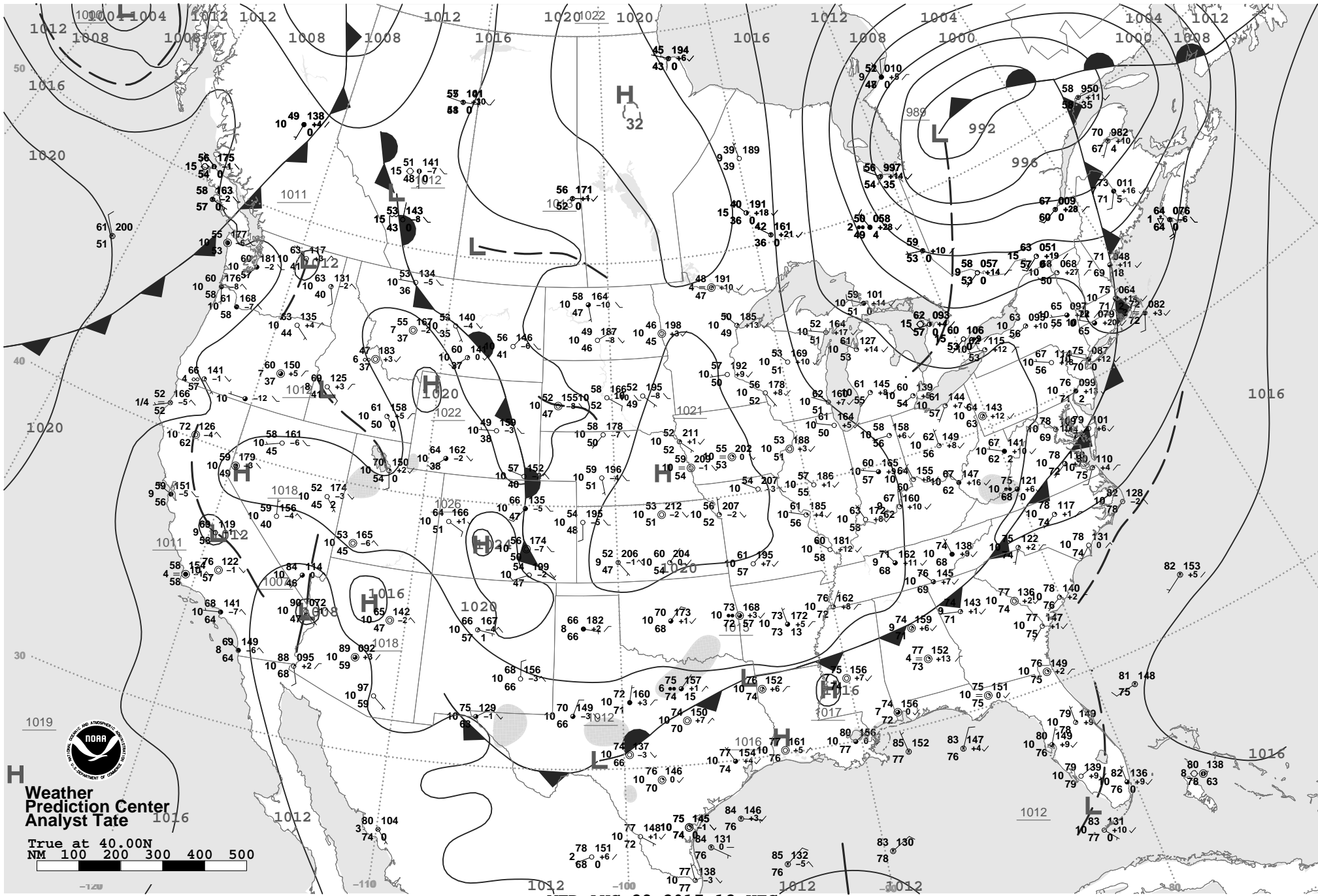
WED AUG 23 2017 12 UTC Surface Weather Map and Station Weather
